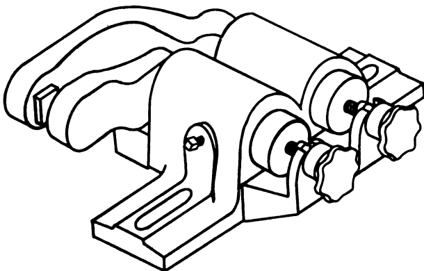
Figure 8-1. Headsaw guide.
